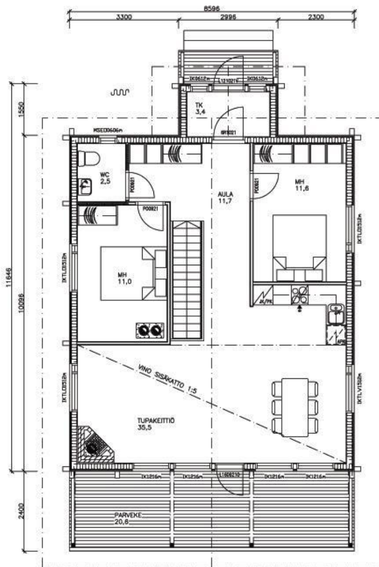
1. KRS 1:50
